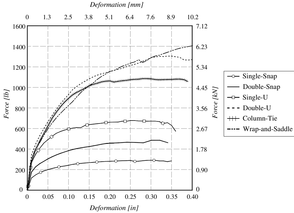
Figure 3.23: Average Normal Translation ( \Delta x ) response of Tie Wire Connections made by Experienced Iron worker
