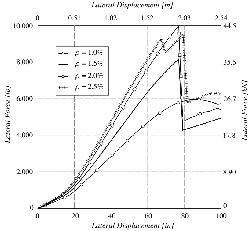
Figure AII.22: Response of Rebar Cage Models with #11 Braces, Height = 40-ft and Diameter = 4-ft
