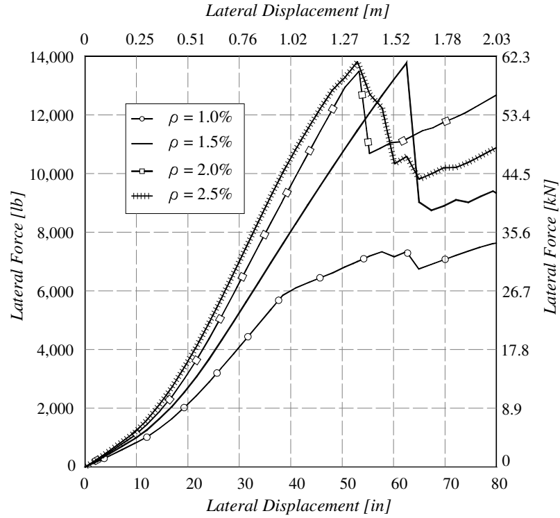
Figure AII.27: Response of Rebar Cage Models with #11 Braces, Height = 50-ft and Diameter = 8-ft
