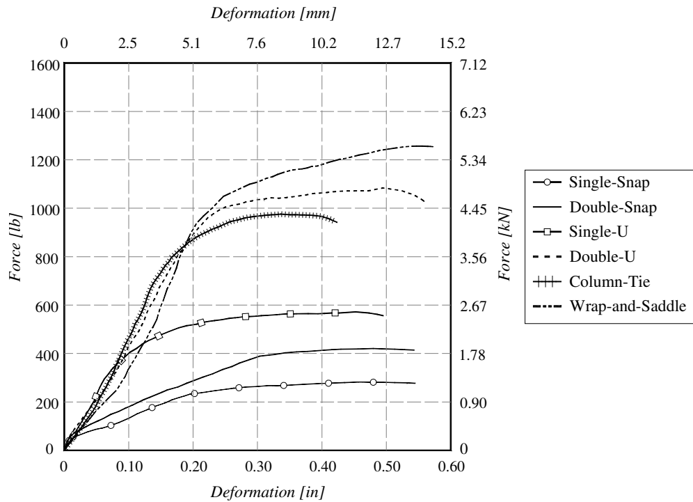
Figure 3.24: Average Normal Translation ( \Delta x ) response of Tie Wire Connections made by Inexperienced Worker
