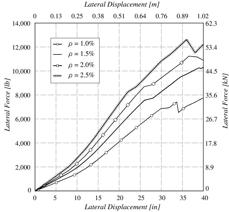
Figure AII.2: Response of Rebar Cage Models with #8 Braces, Height = 30-ft and Diameter = 6-ft
