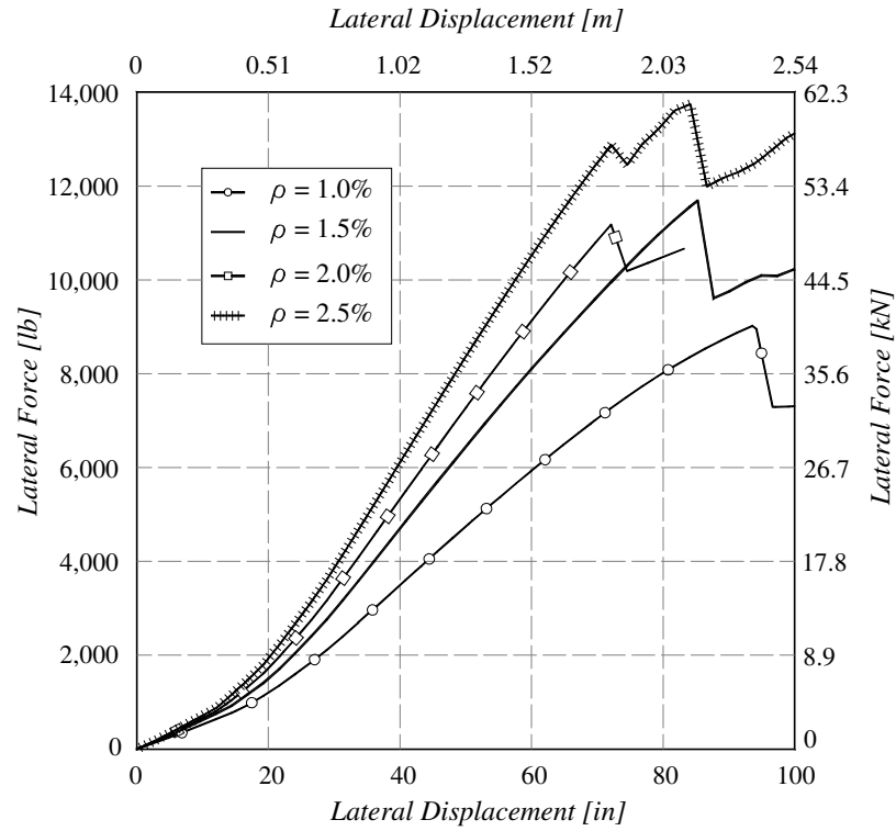
Figure AII.26: Response of Rebar Cage Models with #11 Braces, Height = 50-ft and Diameter = 6-ft
