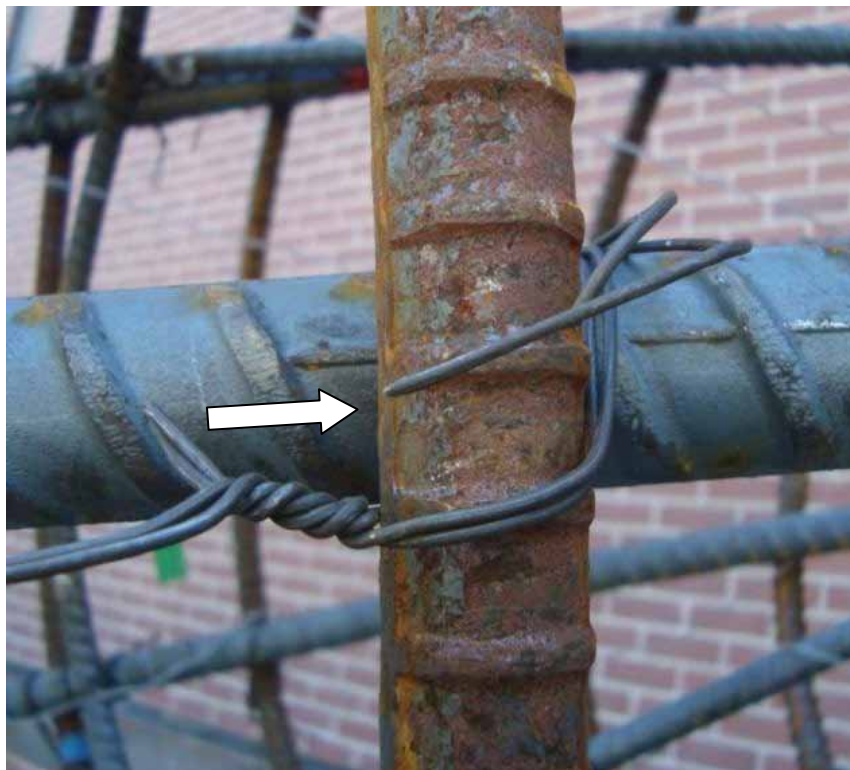
Figure 3.72: Failed Quadruple-snap tie
