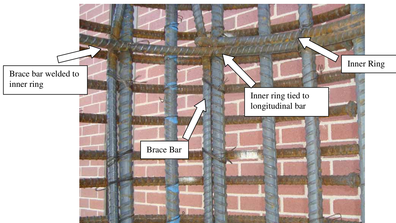
Figure 2.30: Close-up of the Connection Between the end of Braces to the Longitudinal Bar
