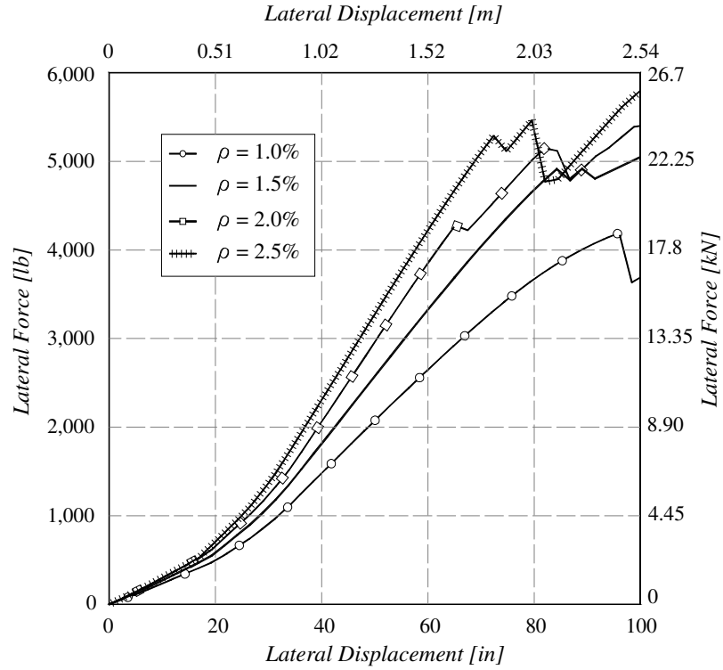
Figure AII.7: Response of Rebar Cage Models with #8 Braces, Height = 50-ft and Diameter = 4-ft
