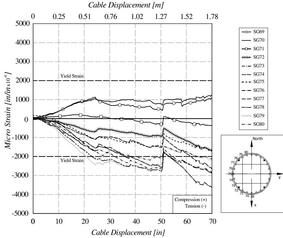
Figure 3.95: Strains at the Top of the Bottom Brace of Specimen II (SG69-SG-80)
