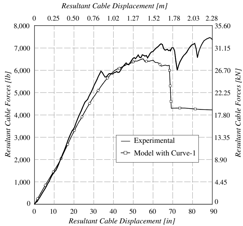
Figure 4.21: Response of Specimen II using Curve-1 for Vertical Springs ( \Delta z ) in the Bracing Elements Boundary Condition
