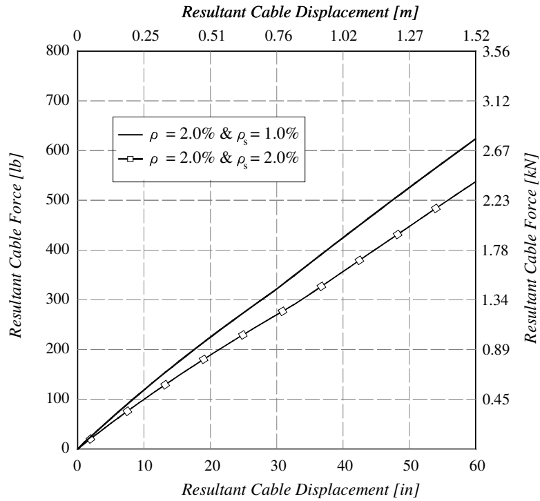
Figure 4.41: Response of Column Rebar Cages without braces and Transverse Reinforcement Ratio equal to 1% and 2%
