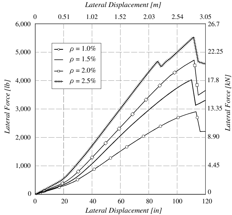
Figure AII.32: Response of Rebar Cage Models with #11 Braces, Height = 70-ft and Diameter = 6-ft
